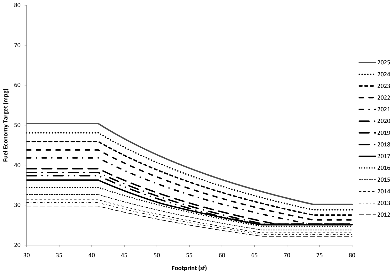
Chart A.2: CAFE Target Curve for Light Trucks
